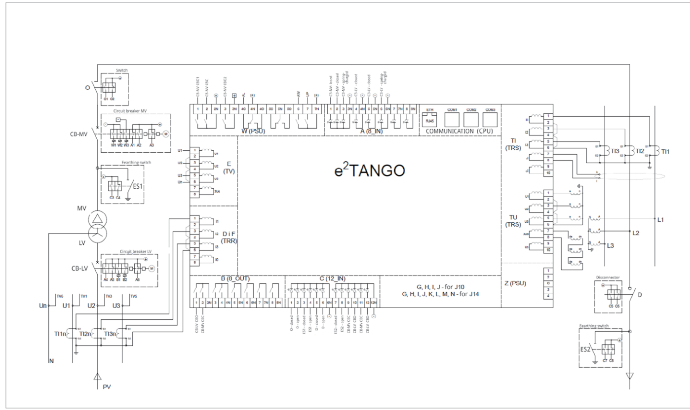
Fig. 3. Application diagram of the e 2 TANGO protection relay that performs protection functions, measurements of current and voltage, control – both on the MV and LV side of the transformer
