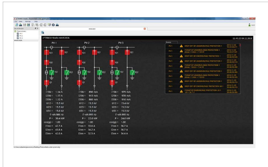
Fig. 4. View of the e2TANGO-Studio engineering software window with the miniSCADA functionality for PV power plants running
