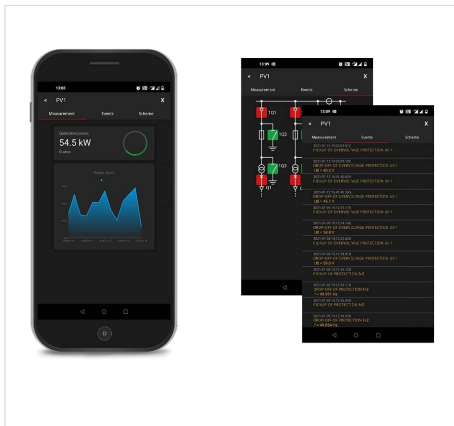
Fig. 5. View of the phone running the miniSCADA window application for a PV solar power plant
